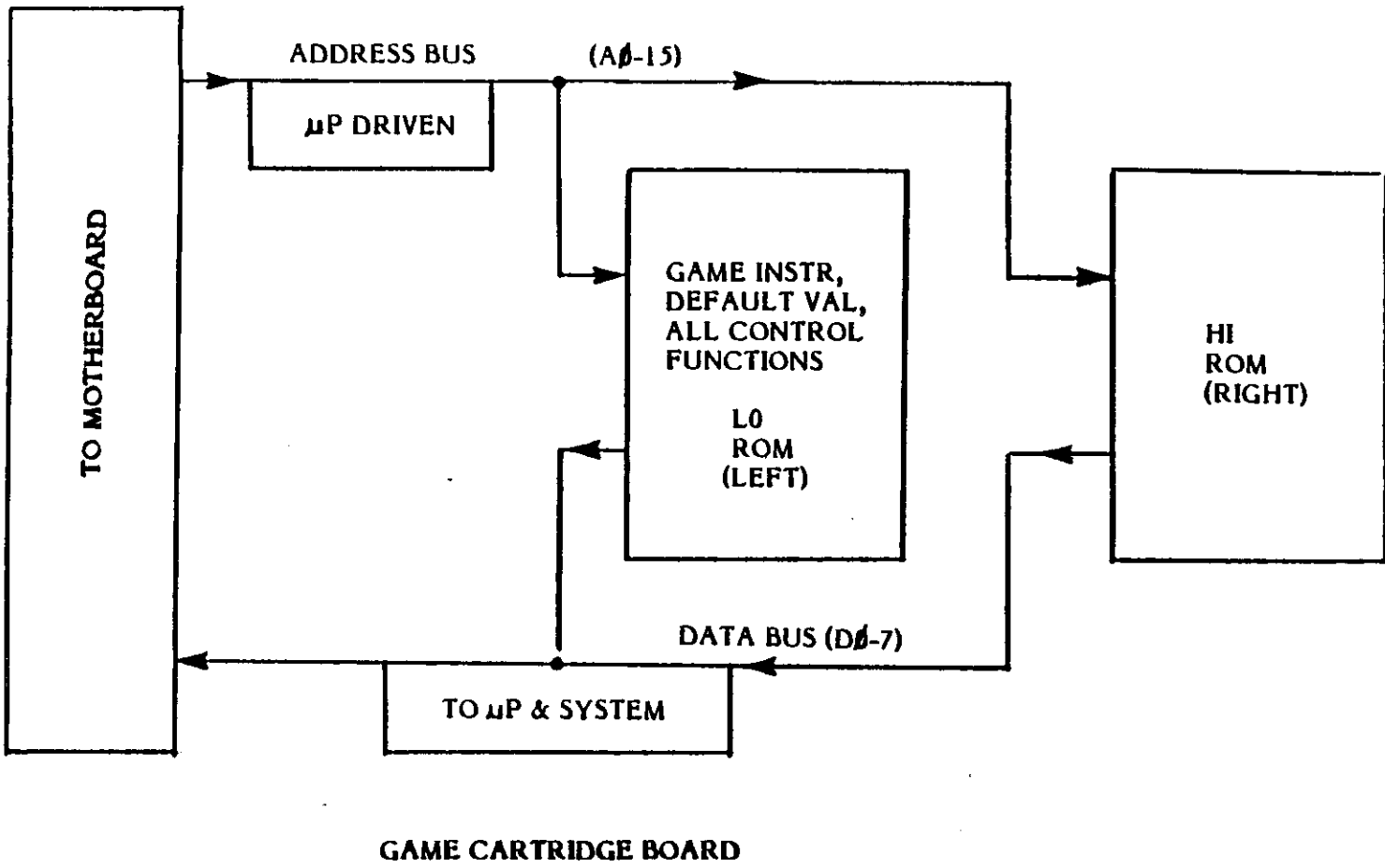
Figure 1-16. Game Cartridge Flow Diagram
