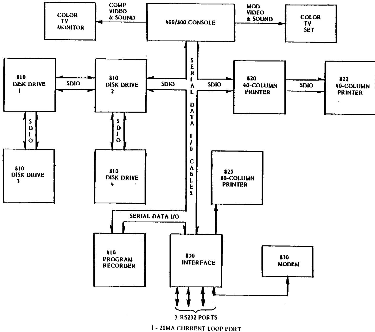
Figure I-17. ATARI Home Computer System Block Diagram
